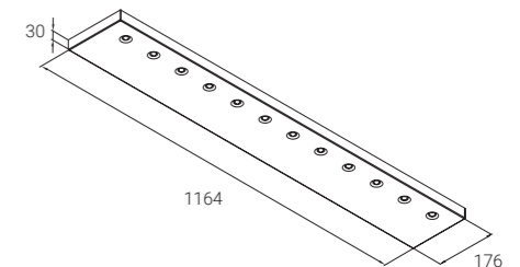
Multicone Rectangular 12 W
