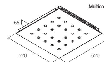
Multicone Panel 24 F
